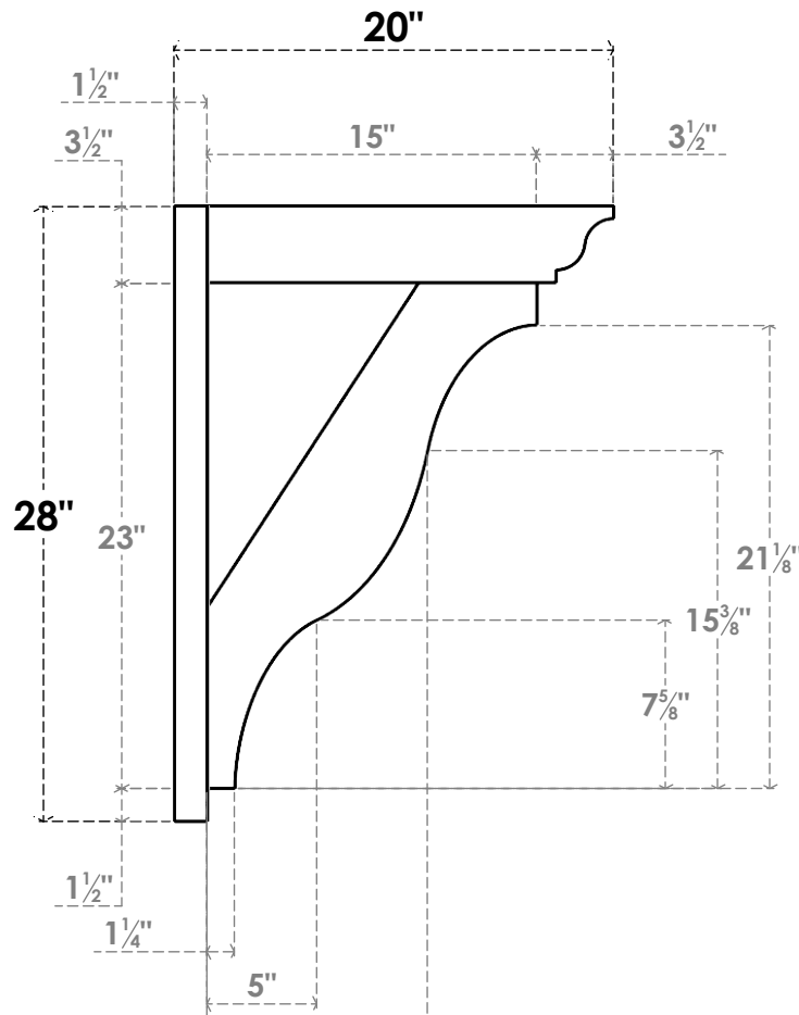
SIDE PROFILE
